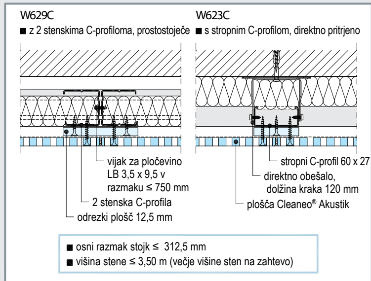
W629C-VO20 Stik s stropom - 2 stenska C-profila
