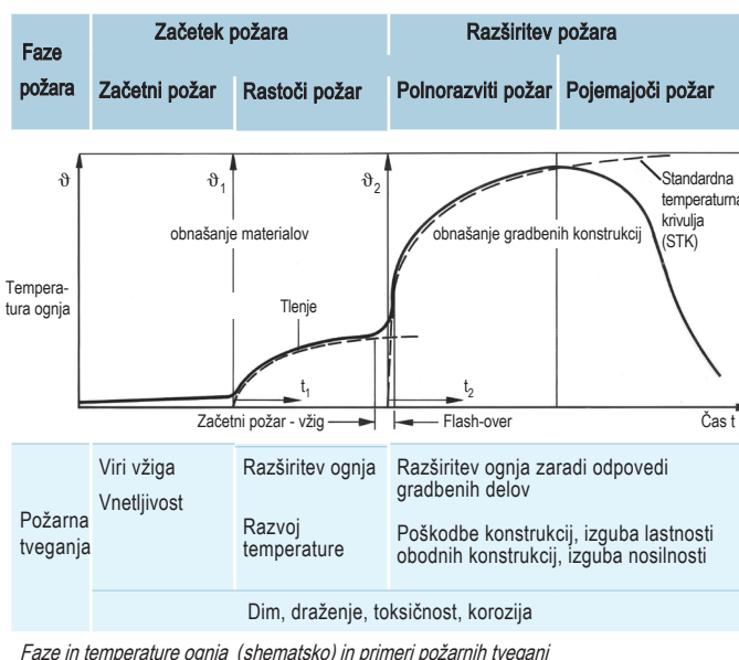
Faze in temperature ognja (shematsko) in primeri požarnih tveganj
